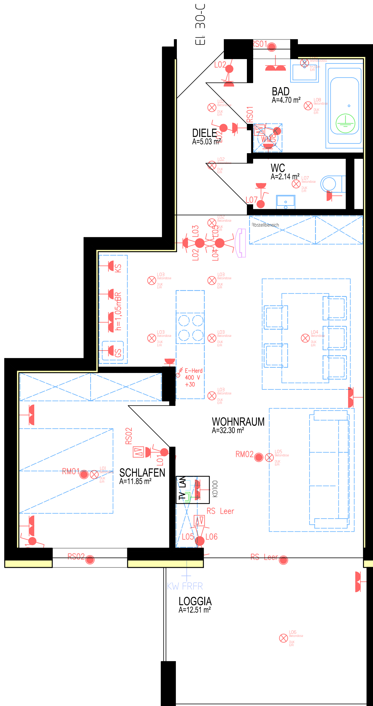
W03 NFL 55,97 m 2 + 12,51 m 2 Loggia
